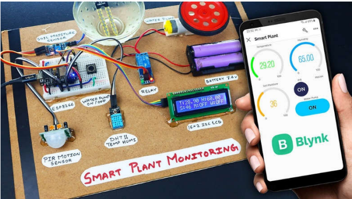
Fig 13: Hardware Design
